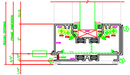
202 I.G. SILL SERIES 403X - 2" X 4 1/2" SHEARBLOCK
